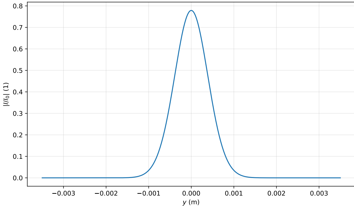
Intensity profile I(x=0, y, z=1.194)/I_0 , \text{Pin}=0.1\text{Pcr} , artificial time
